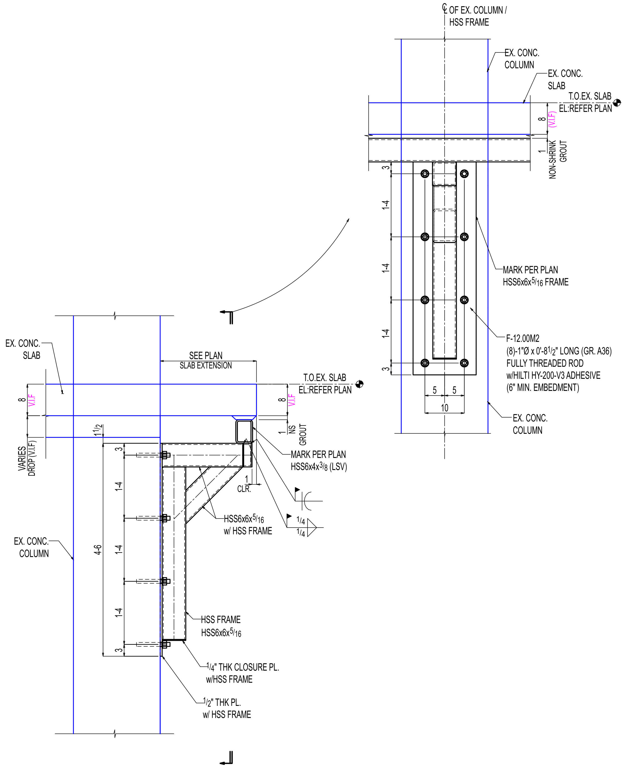
N-N E-12.00 (REF:10/S315) OTHERS NOT SHOWN FOR CLARITY
