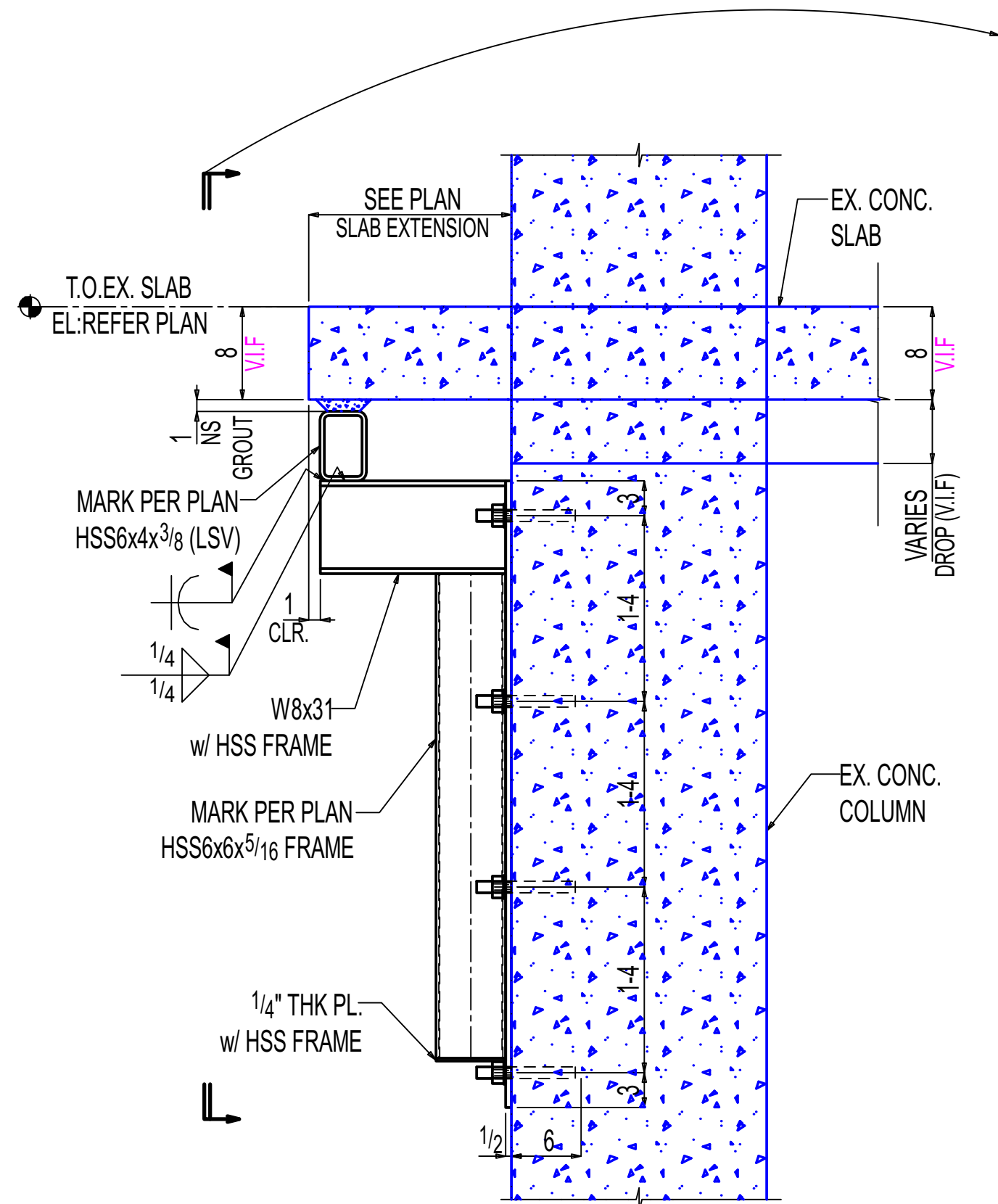
L-L E-12.00 (REF: 10/S315) OTHERS NOT SHOWN FOR CLARITY
