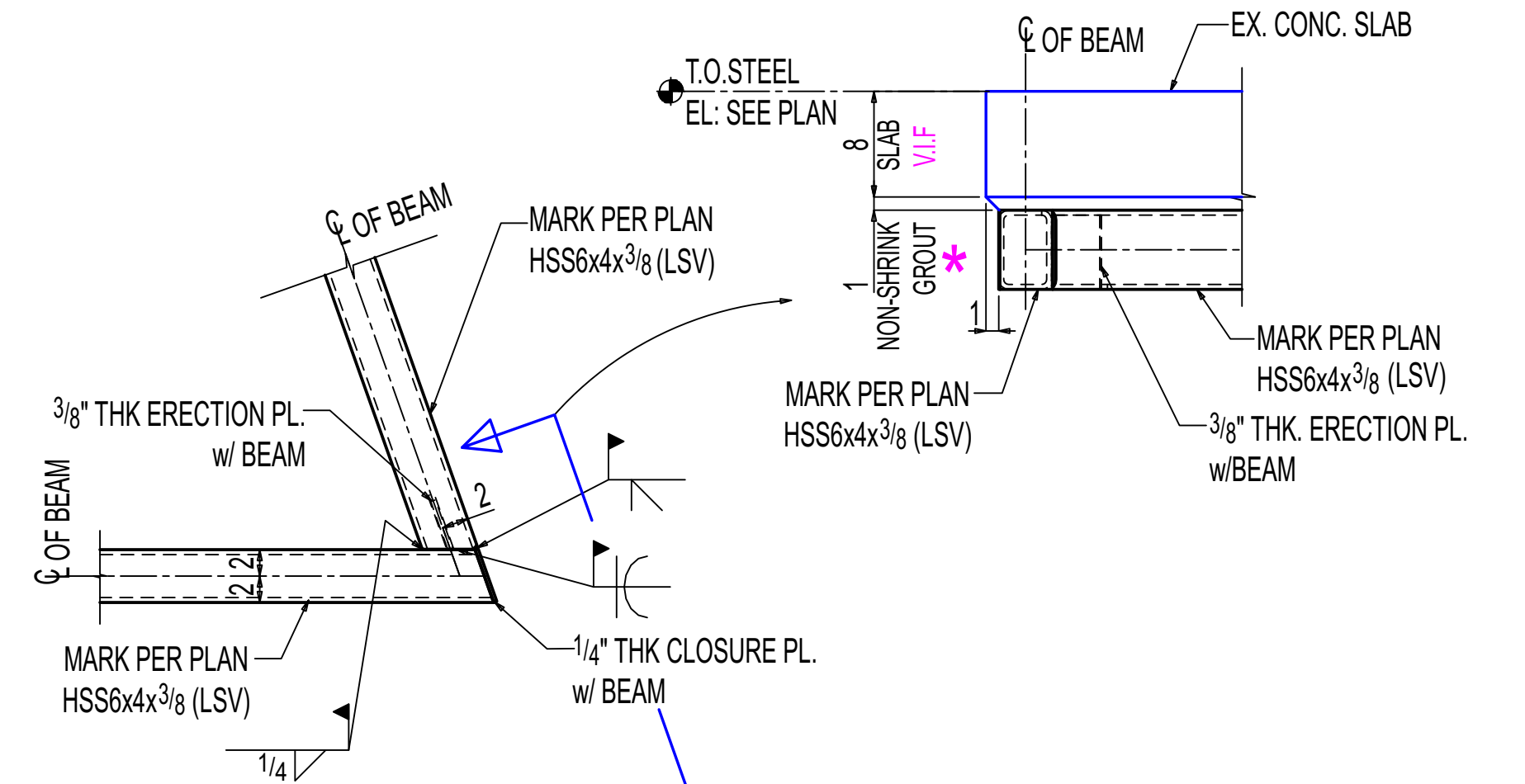
DETAIL-3 E-10.00 OTHERS NOT SHOWN FOR CLARITY
