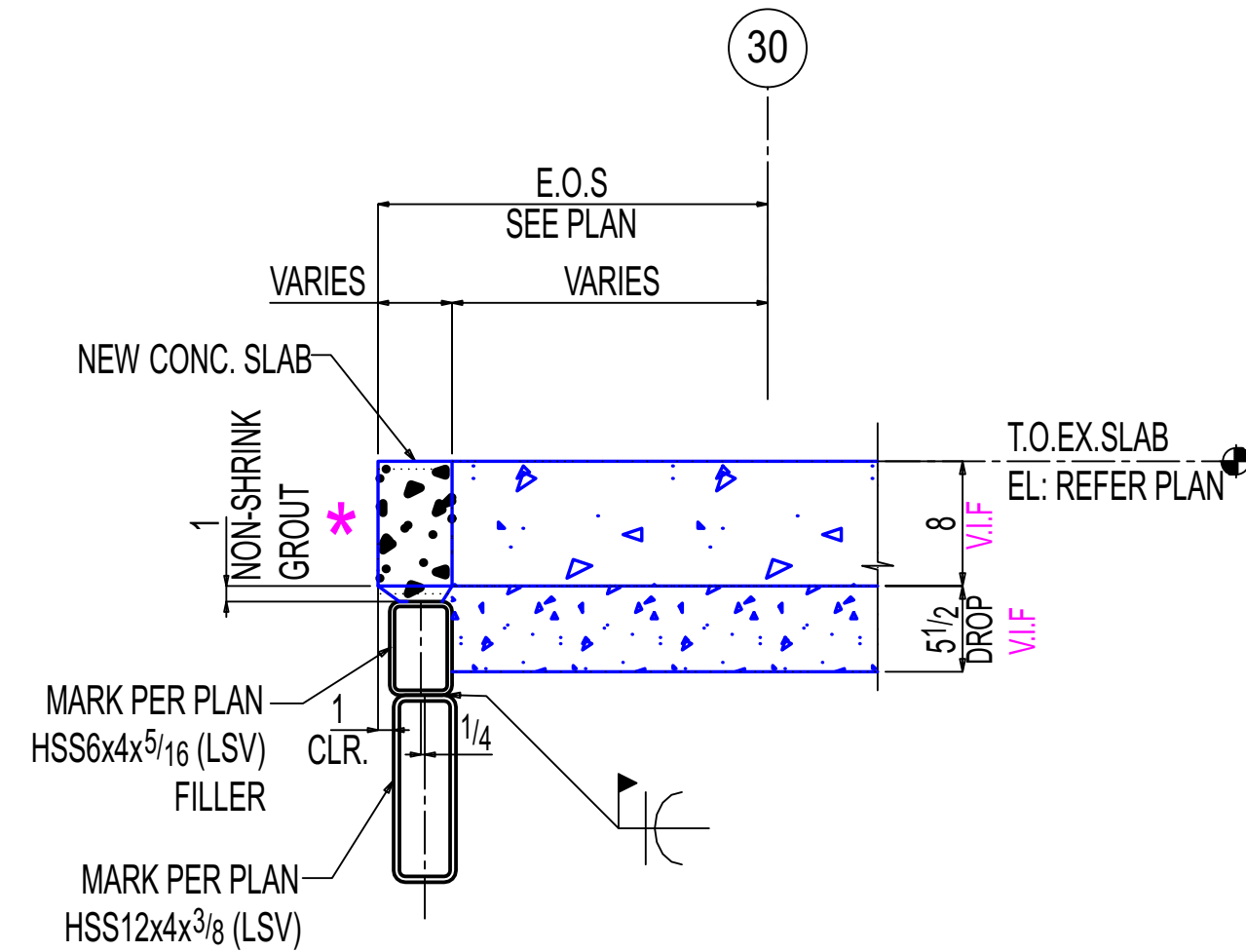
M-M E-12.00A (REF: 4/S315) OTHERS NOT SHOWN FOR CLARITY
